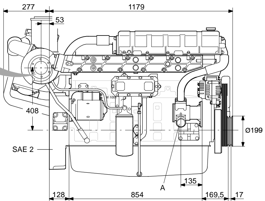
Exhaust outlet flange 8368 64433
