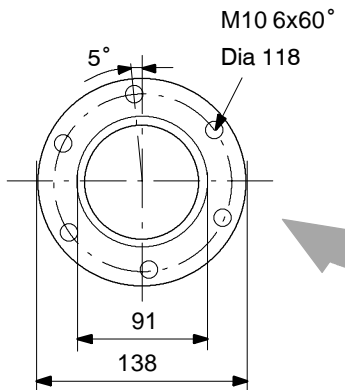
Exhaust outlet flange 8368 64433
